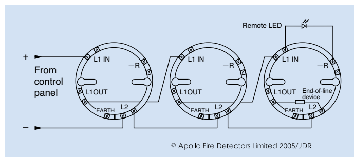
Fig.5 Schematic wiring diagram of Series 65 monitored detector circuit
