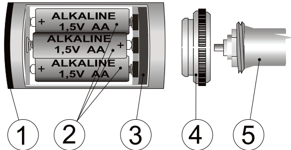
Fig. 1: 1 – indicator; 2 – battery; 3 – safety ring; 4 – adapter; 5 – radiator valve
