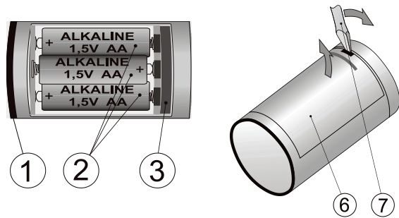
Fig. 3: 1 – indicator; 2 – battery; 3 – safety ring; 6 – battery cover; 7 – auxiliary tool (a screwdriver);
