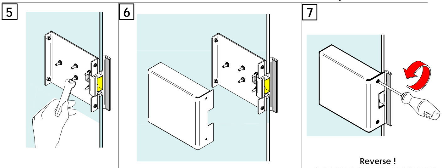
Adjustable cover latch
