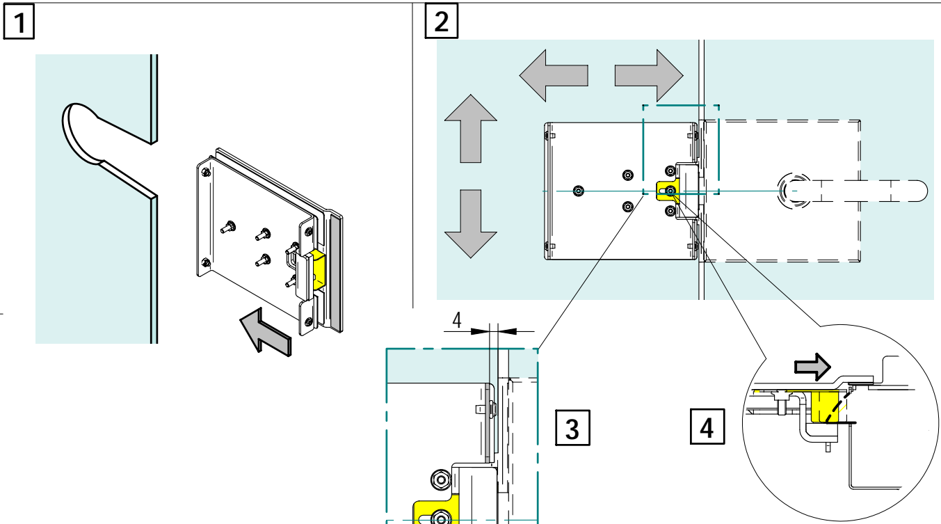
Adjustable cover latch
