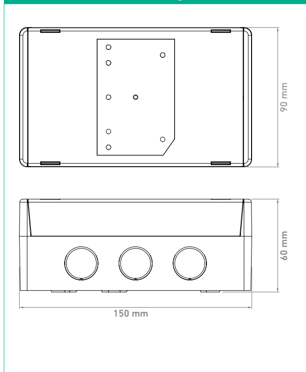
Figure 1: Intelligent Twin Switch Monitor dimensional drawing
